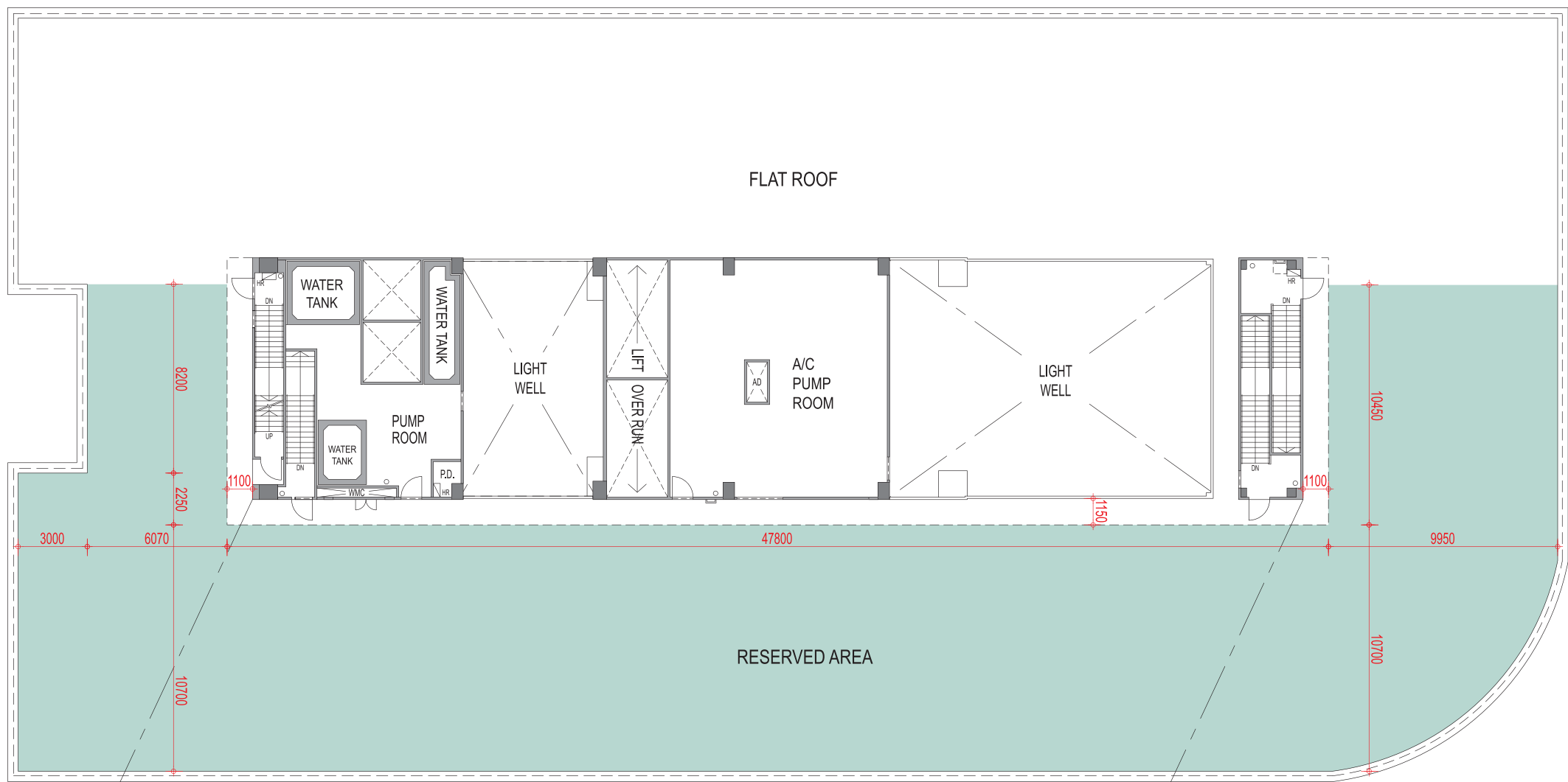
ROOF PLAN
