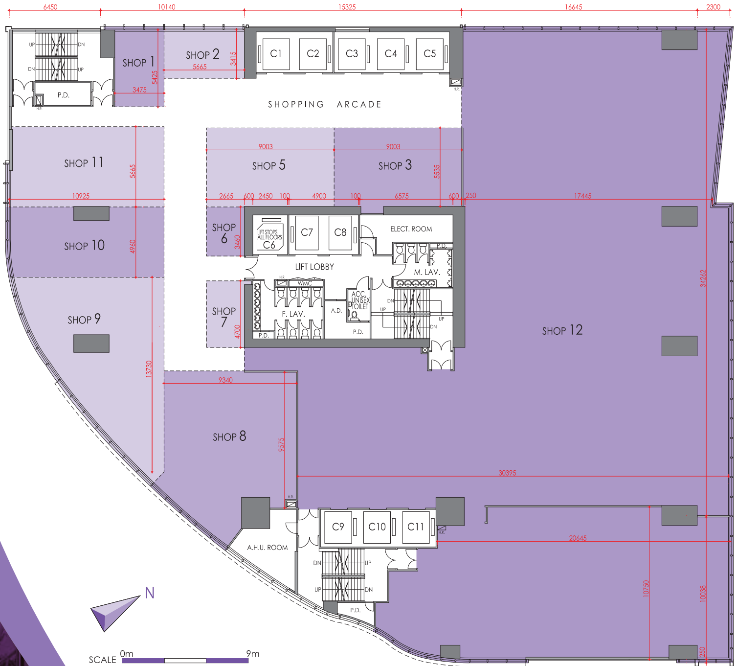
11 th Floor Area Schedule
