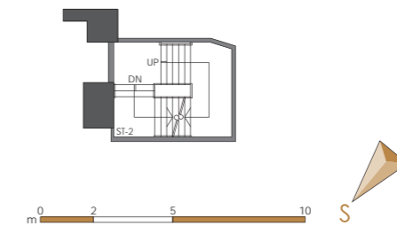
PART PLAN OF STAIRCASE 2 BETWEEN G/F & 1/F
