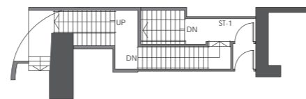
PART PLAN OF STAIRCASE 1 BETWEEN 2/F & 3/F
