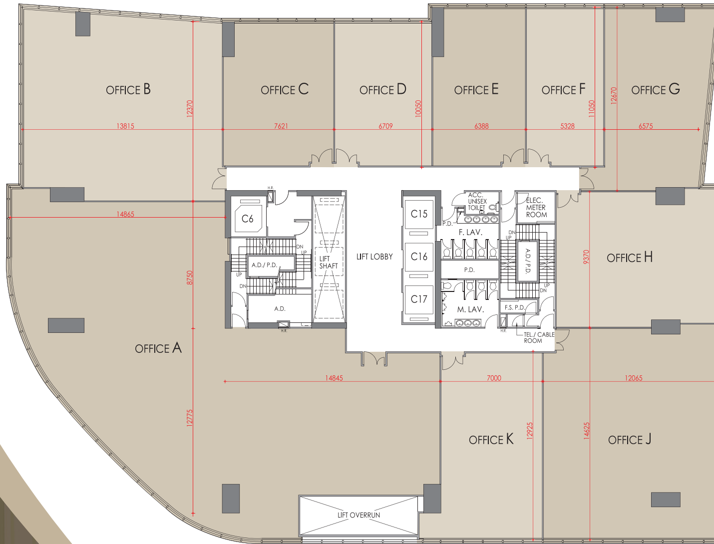
21 st Floor Area Schedule
