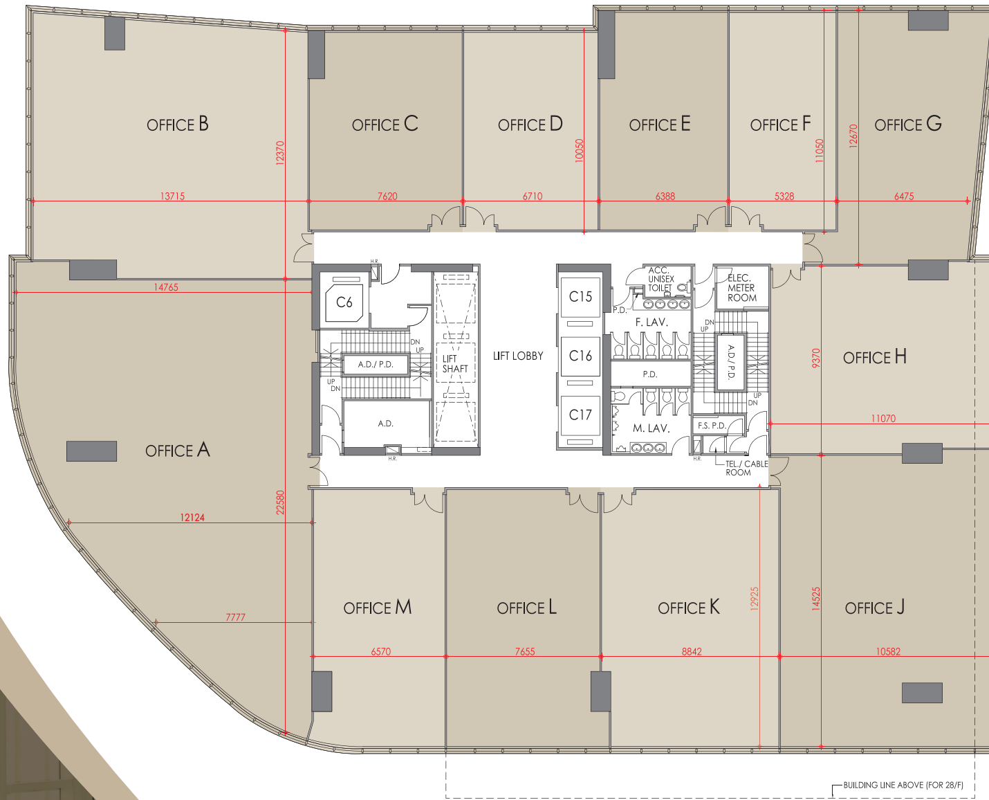
26 th & 28 th Floor Area Schedule
