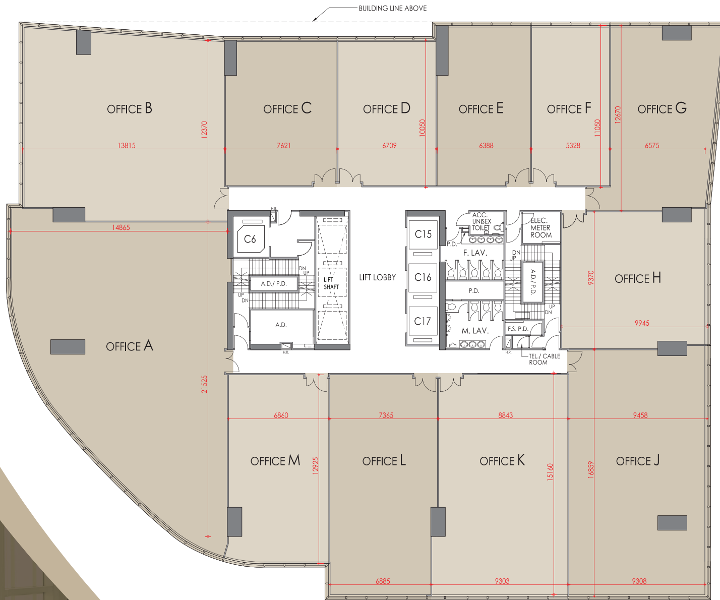
30 th Floor Area Schedule
