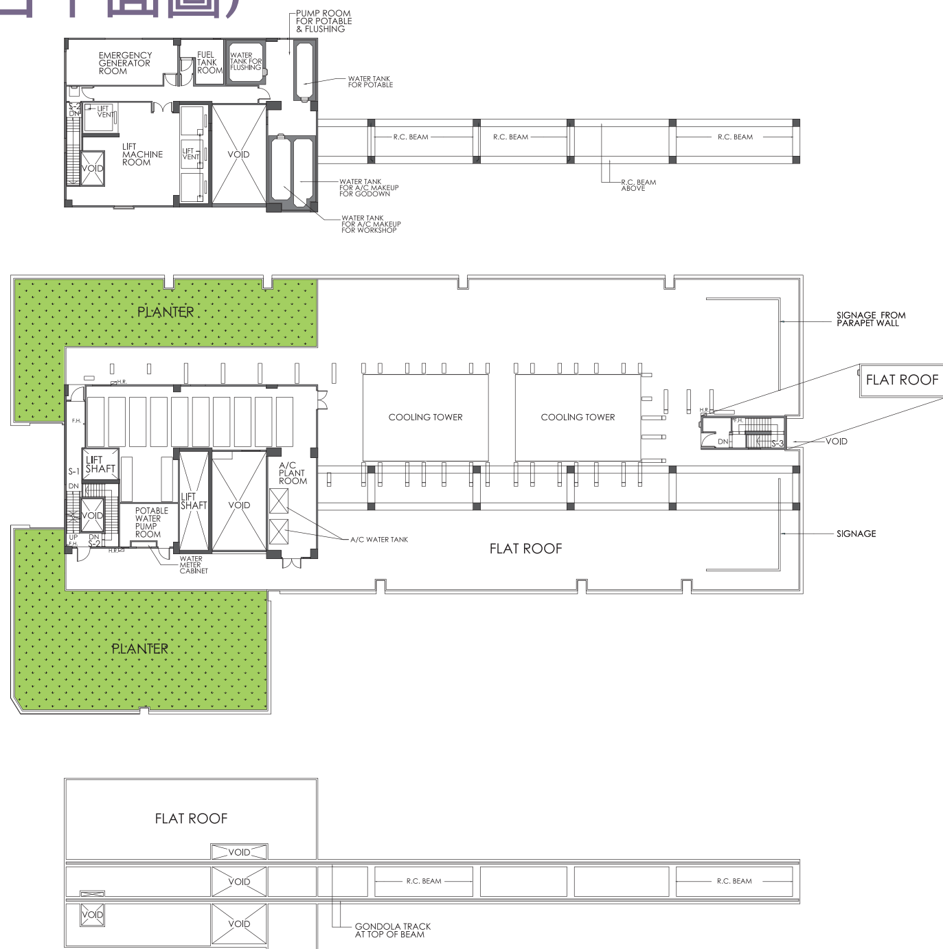
UPPER ROOF PLAN (上層天台平面圖)
