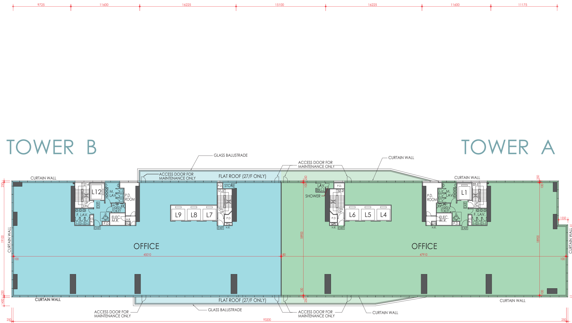
27th -30th Floor Area Schedule (Tower B)
