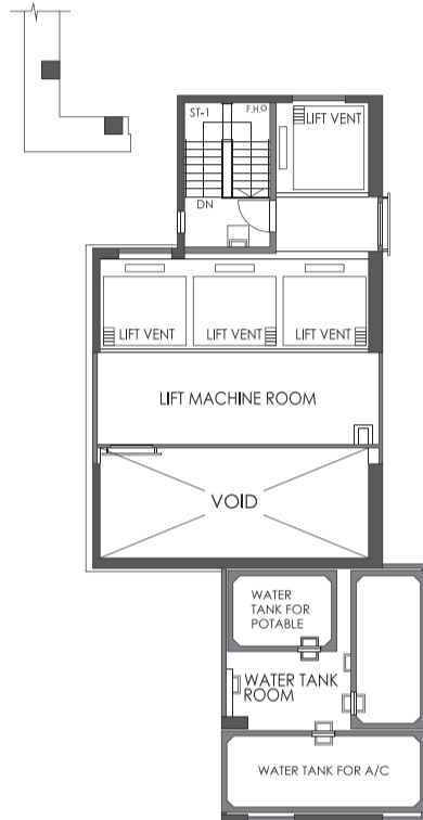
UPPER ROOF PLAN
