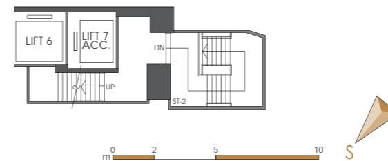
PART PLAN OF STAIRCASE 2 BETWEEN 1/F & 2/F
