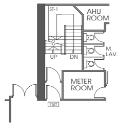
PART PLAN OF 10/F
