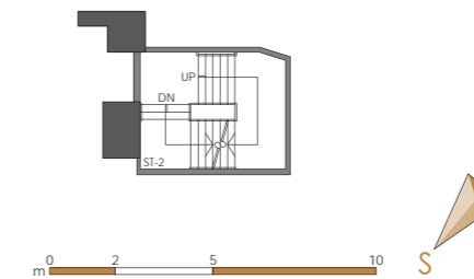
PART PLAN OF STAIRCASE 2 BETWEEN G/F & 1/F
